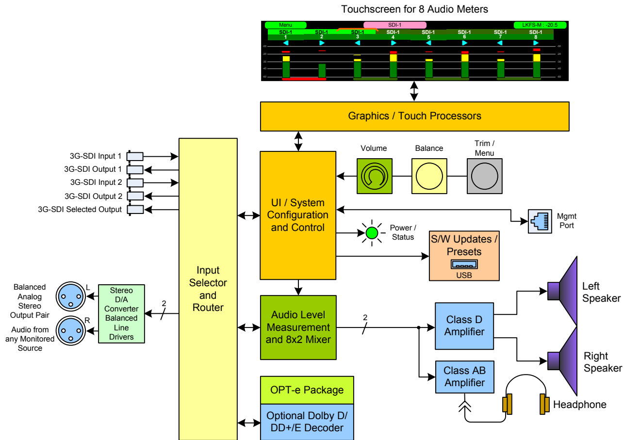
Figure 3-1: eAMP1-8M Block Diagram
